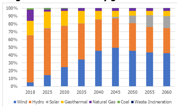
Figure 3: Tūi electricity generation
